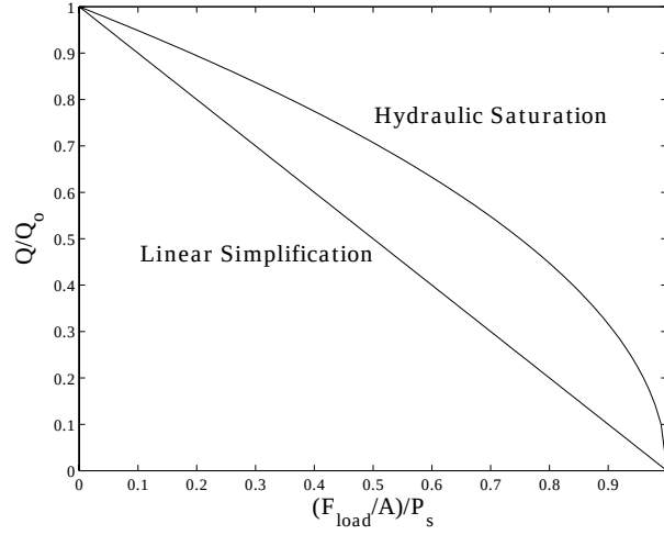
Figure 4-4: [SIM] The power saturation profile for a hydraulic servo valve is a square root relationship between flow and pressure. In order to understand the effects of saturation on the actuator through linear analysis, a linear saturation relationship is assumed. The linear profile is a worse case than the square root saturation.
