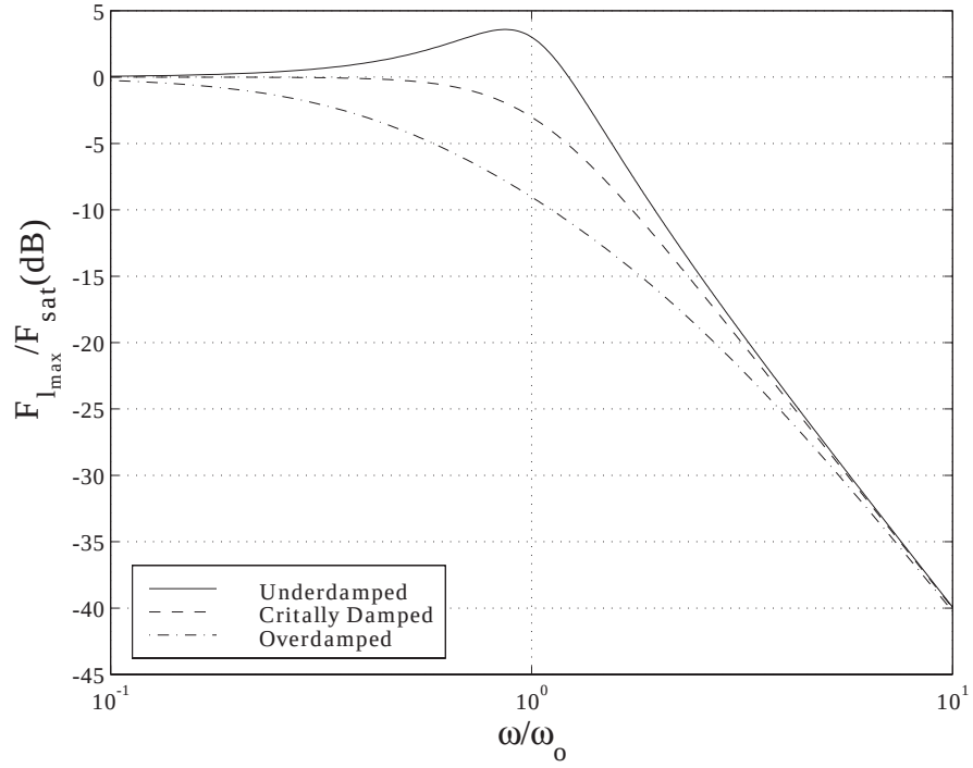
Figure 5-6: SIM EM large force bandwidth due to force and velocity saturation. The motor mass spring resonance \omega_o defines the large force bandwidth of the actuator. The B group (generalized damping) defines the shape of the profile around the saturation frequency. The three lines represent underdamped, critically damped, and overdamped frequency response. This plot only represents the large force capabilities of the actuator with the load fixed.
