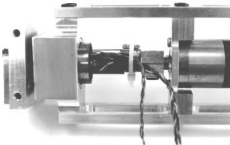
Figure 5-13: Closeup of spring
