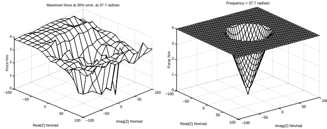
Fig. 12. Maximum output force vs. load impedance at 38 rad/sec
