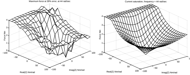
Fig. 13. Maximum output force vs. load impedance at 44 rad/sec
