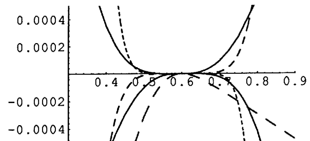
Figure 1. Deviations of expansions from exact linear orbit
