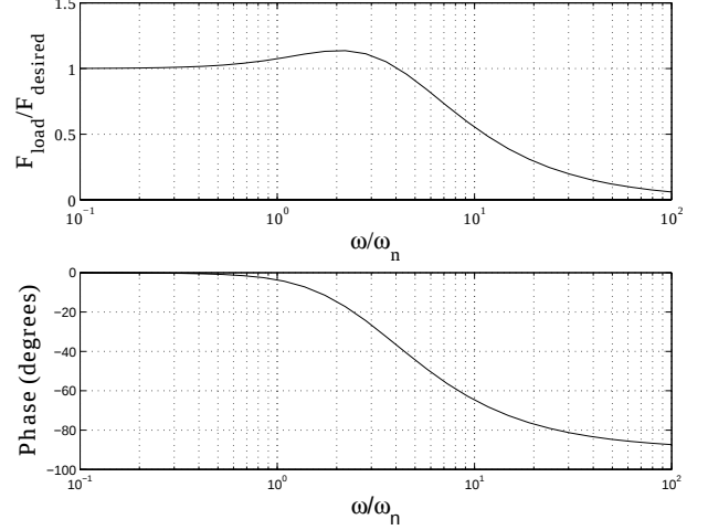
Fig. 4. This is a bode plot of the closed loop system. \Omega = 3 and \zeta_c = 1 .
