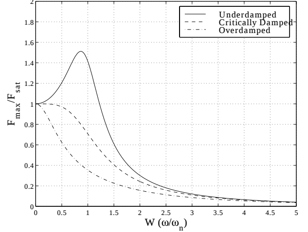
Fig. 3. The B group (generalized damping) defines the large force bandwidth of the actuator. The three lines represent underdamped, critically damped, and overdamped frequency response.
