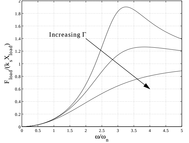
Fig. 6. The impedance of the actuator at low frequency is zero and is k_s at high frequency. In this example \Omega = 3 . As \Gamma is increased there is an effective reduction in the impedance at the controlled natural frequency.
