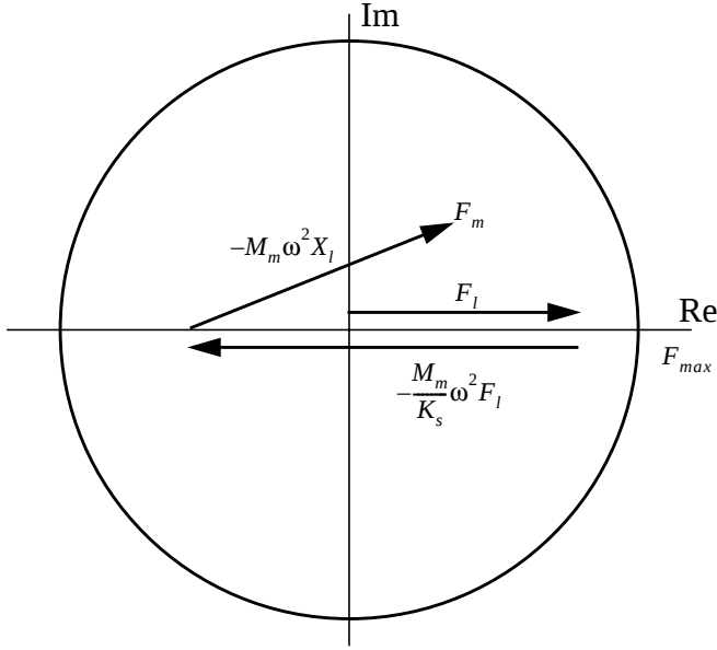
Figure 5: Phase Diagram of Necessary Motor Force
