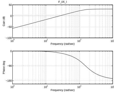
Figure 10: Theoretical Bode Plot of Output Impedance
