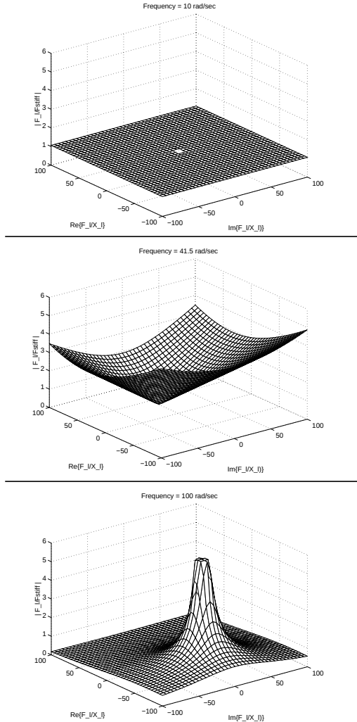
Figure 7: Plot of F_l / F_{stiff} vs. Z
