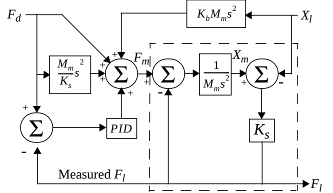
Figure 8: Control Architecture
