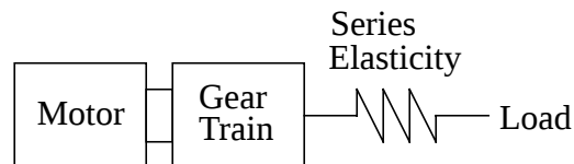
Figure 1: Block Diagram of Series-Elastic Actuator
