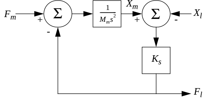
Figure 3: Frequency Domain System Diagram
