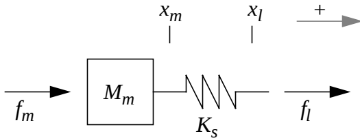
Figure 2: Model of a series-elastic actuator
