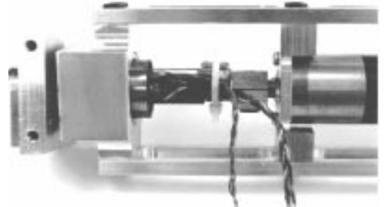
Figure 12: Mounting of Strain Gauges on Series Spring
