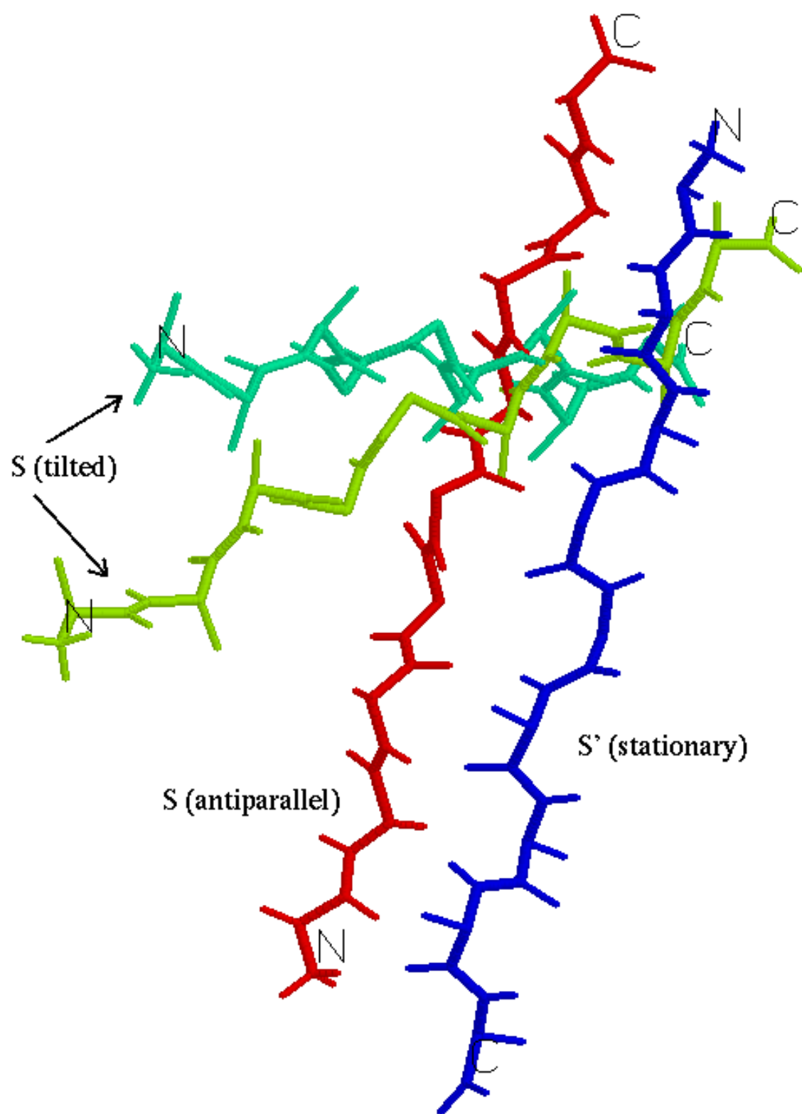
Figure 15: 3 packing solutions to constraint set B .
