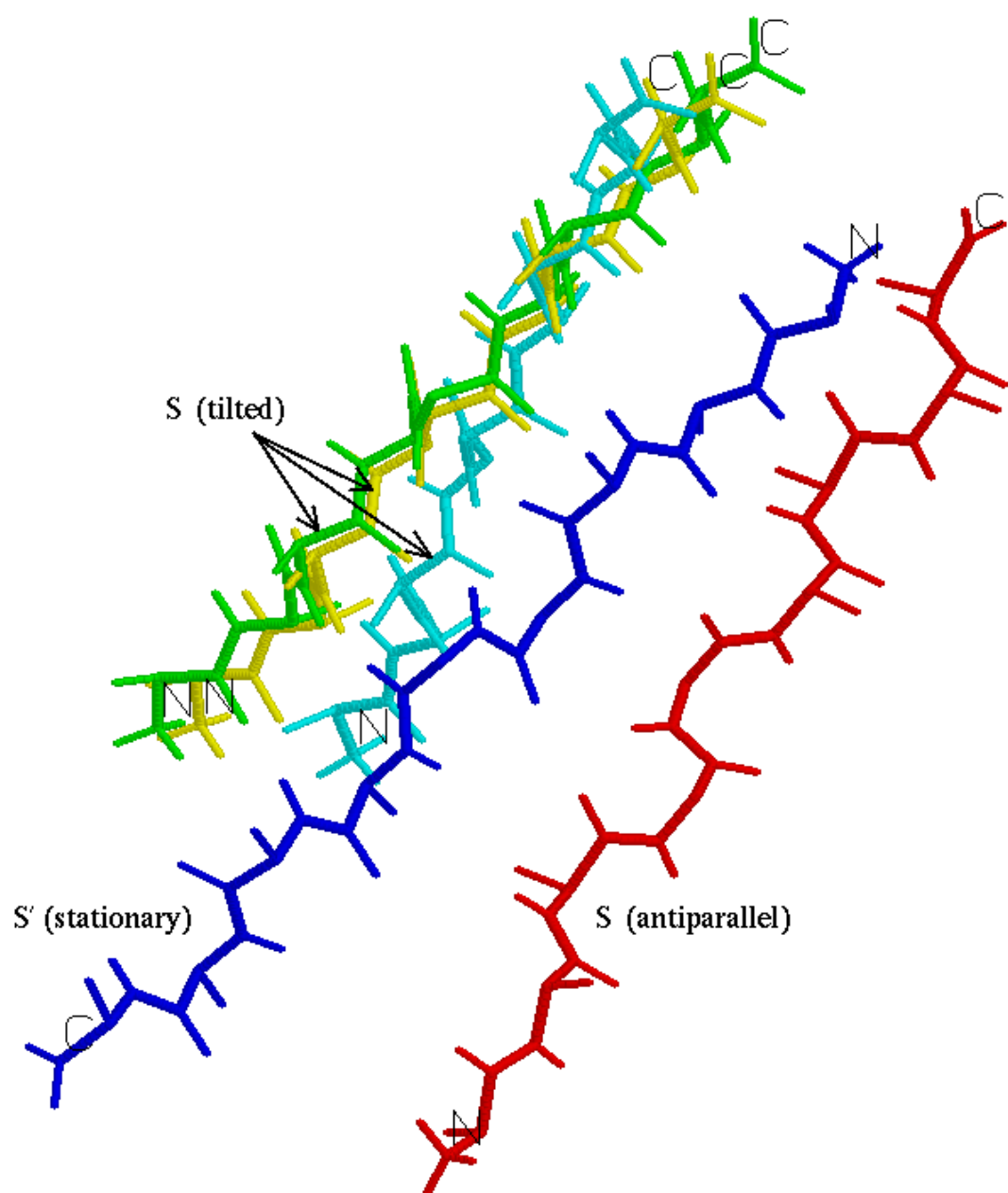
Figure 14: 4 packing solutions to constraint set A .
