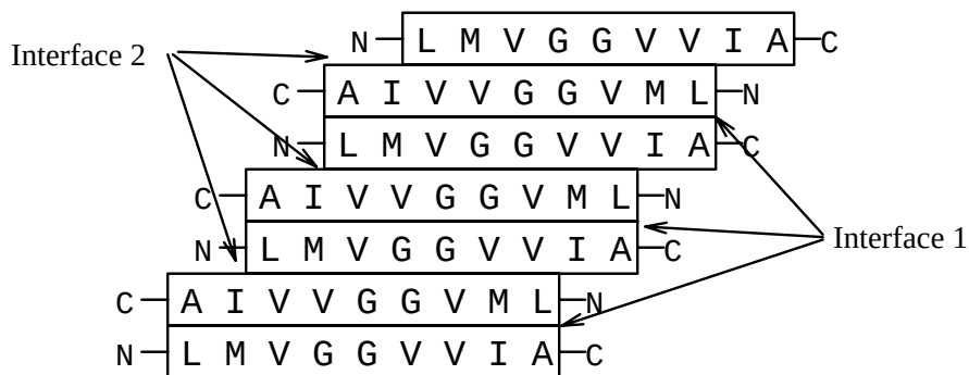
Figure 2: Structure of \beta amyloid fibril proposed by Lansbury et al. [8]
