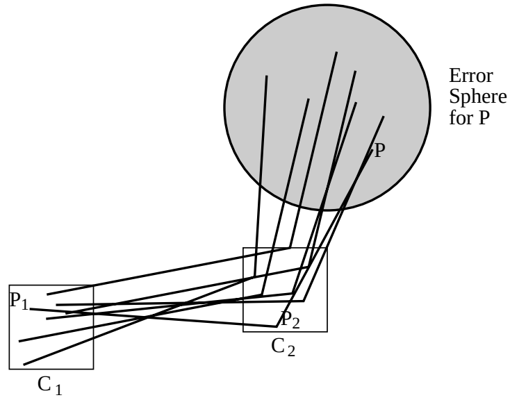
Figure 4: The error spheres for points in S when the P_i are constrained to be somewhere within cubes contained in spheres centered on Q'_i . Illustrated here in two dimensions.
