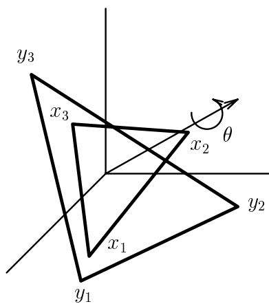
Figure 6: When two triangles are coplanar and their centroids are coincident, there is only one angle of rotation, \theta , to determine.
