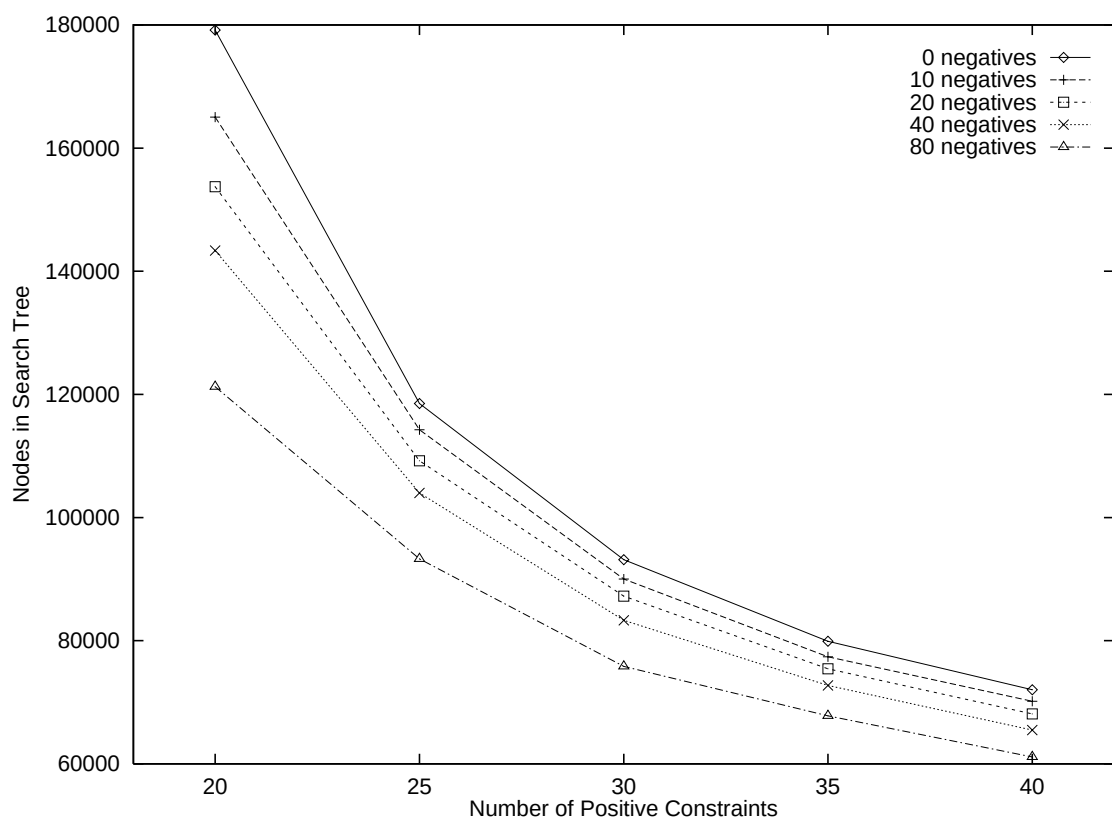
Figure 12: Computational resources used by various combinations of positive and “near-miss” negative constraints.
