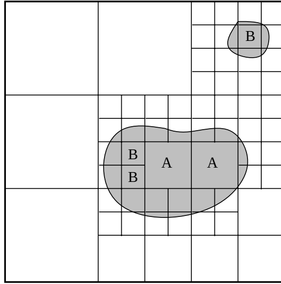
Figure 8: Solutions will generally be clustered into regions (shown shaded) in a high-dimensional space, characterized by the placements of the P_i . Each leaf of the search tree maps into some rectangular region in this space whose size is determined by the resolution. AmbiPack samples one point (or at most a few) for each leaf region in this solution space. At a coarse resolution, only leaves completely inside the shaded solution region are guaranteed to produce a solution, e.g. the regions labeled A. As the resolution is improved, new leaves may lead to solutions, some of them will be on the boundary of the original solution region containing A, others may come from new solution regions not sampled earlier.
