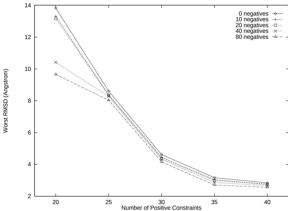
Figure 13: Quality of structures produced by various combinations of positive and “near-miss” negative constraints. The RMSD is measured by applying the computed transforms to one of the P22 tailspike monomers (from the X-ray structure) and measuring the displacement from this monomer to the nearby monomer in the X-ray structure.
