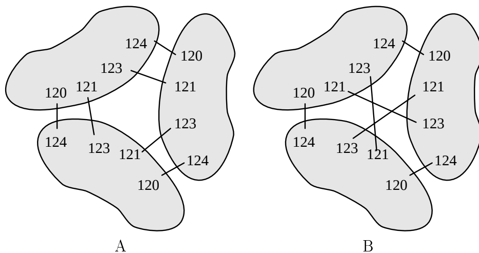
Figure 1: Two ambiguous intermolecular distances can have two different interpretations. The P22 tailspike protein is shown schematically with two different interpretations for the proximity pairs 120–124 and 121–123.
