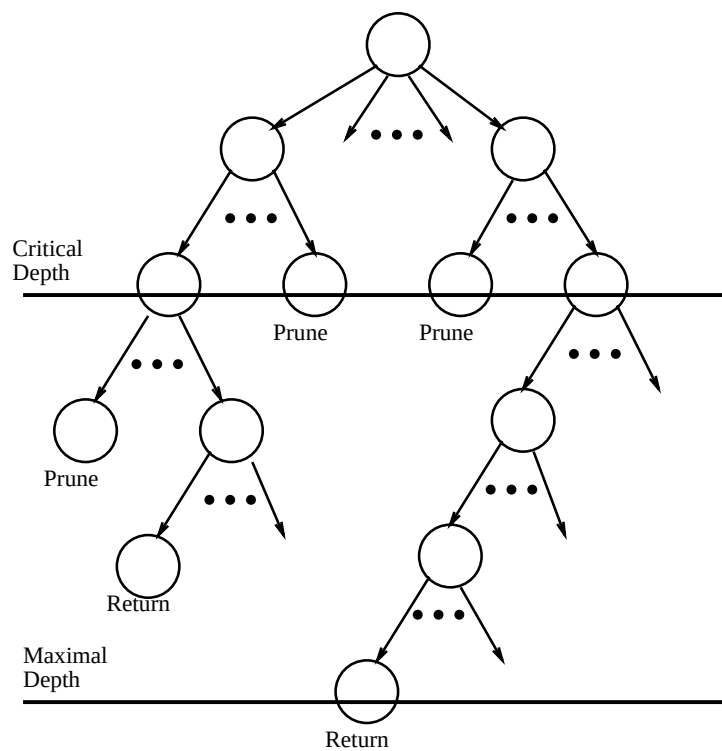
Figure 9: Illustration of the search using a critical depth and maximal depth.
